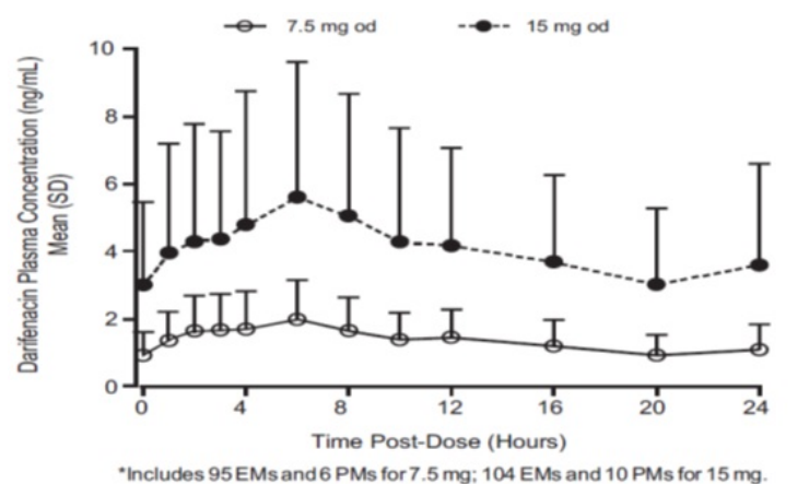
Figure 1: Mean (SD) Steady-State Darifenacin Plasma Concentration-Time Profiles for Darifenacin 7.5 mg and 15 mg in Healthy Volunteers Including Both CYP2D6 EMs and PMs*
